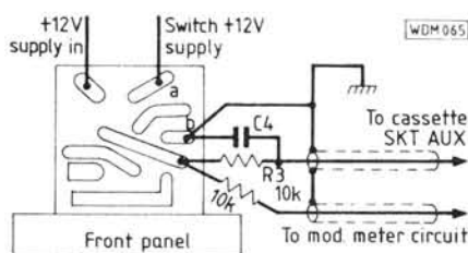
Fig. 4: Connections to volume control p.c.b.
