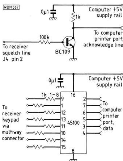
Fig. 6: Circuit for computer interface
