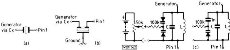
Fig. 7: Component connection points used for resonance testing
