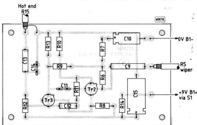
Fig. 4: Full size track pattern and component layout for pre-amplifier p.c.b.
