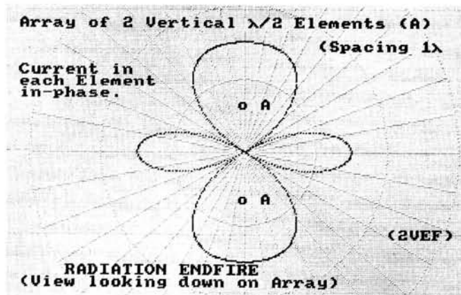
Fig. 4.5: Radiation pattern from a 2 element Endfire array. Element spacing 1 wavelength
