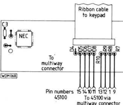
Fig. 7: Control p.c.b. layout showing C3 (scan speed) and connections for parallel computer control of keypad
