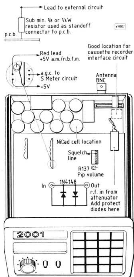
Fig. 1: Internal layout of AR-2001
