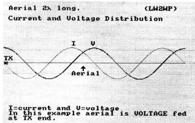
Fig. 4.1: Voltage and current distribution on a linear radiator 2 wavelengths long. (see text regarding harmonic operation)
