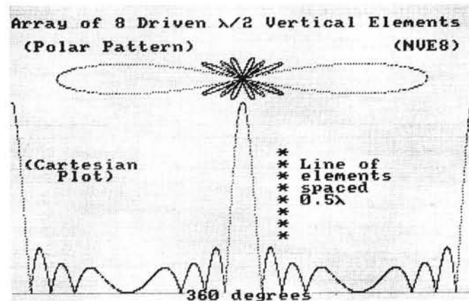
Fig. 4.7: Broadside array of 8 vertical half-wave elements. Polar pattern and Cartesian plot. (See text regarding gain from each main lobe)
