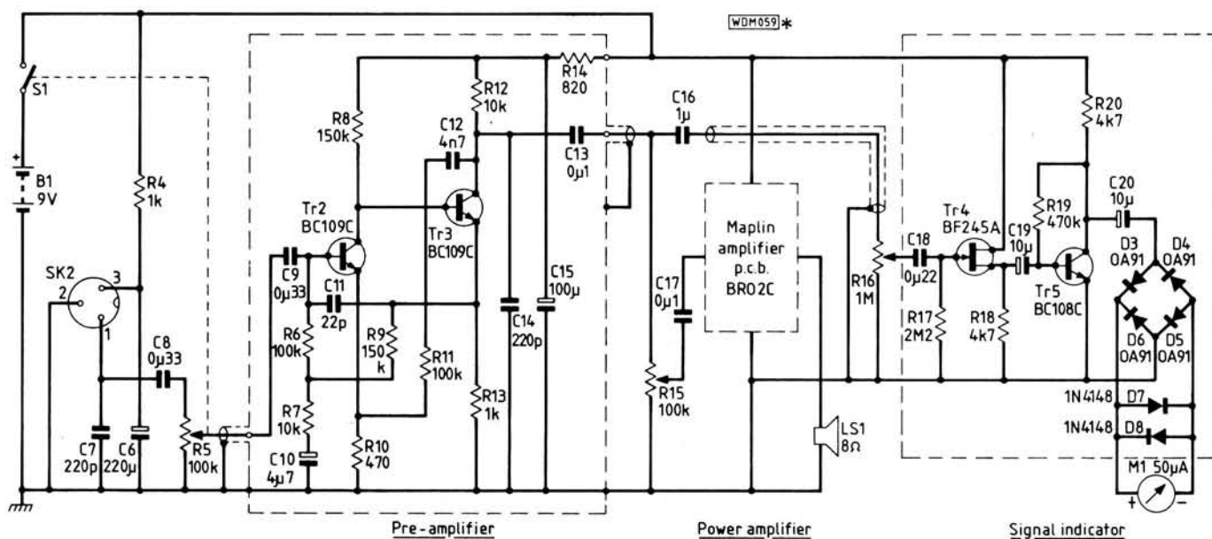
Fig. 1: Circuit diagram of amplifier and indicator
