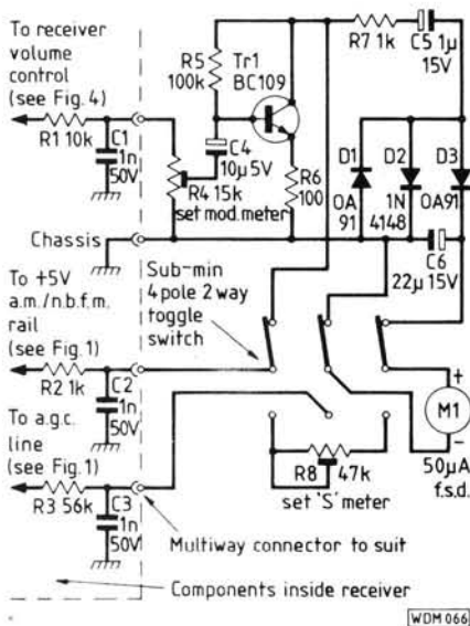
Fig. 5: Signal and modulation meter circuit
