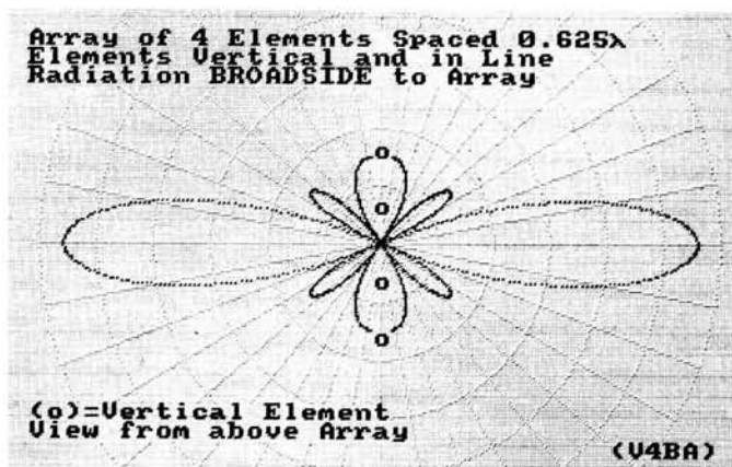
Fig. 4.6: Radiation pattern. Broadside array consisting of 4 vertical half-wave elements
