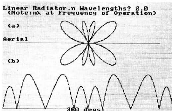
Fig. 4.2: (a) Polar pattern. Radiation at fundamental frequency of a linear radiator 2 wavelengths long. (b) For same radiator but as a Cartesian plot. (Horizontal mode)
