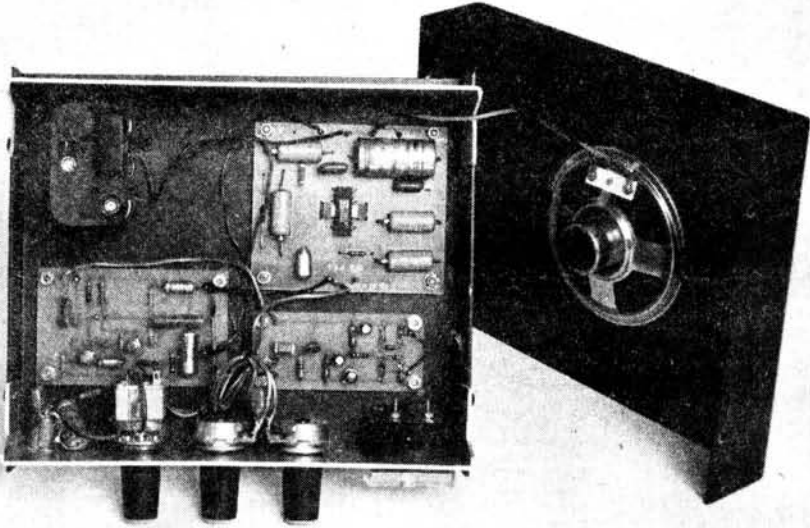
Internal view of prototype. Note all signal paths wired in miniature screened cable
