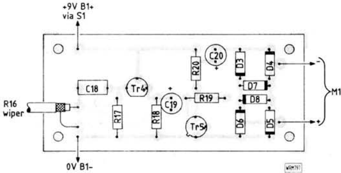
Fig. 5: Full size track pattern and component layout for indicator p.c.b.
