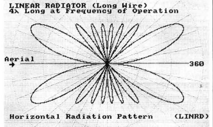
Fig. 4.4: Radiation pattern. Linear radiator 4 wavelengths long. Note number of minor lobes and that main lobes are at a smaller angle to the radiator. (see text)
