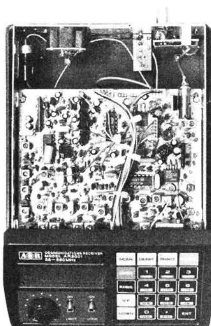
Internal view of unmodified AR-2001
