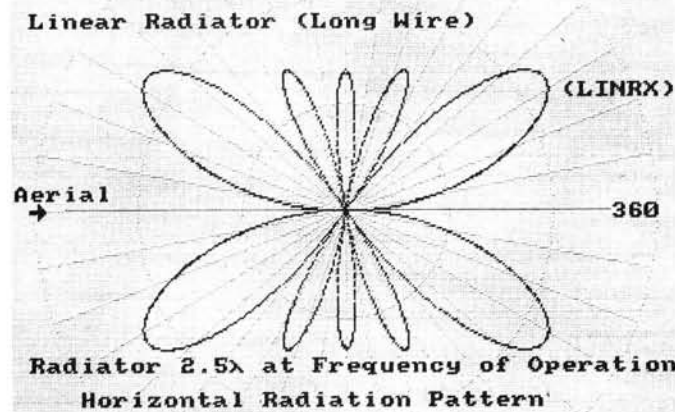
Fig. 4.3: Radiation pattern: Linear radiator 2.5 wavelengths long. Note increase in number of minor lobes
