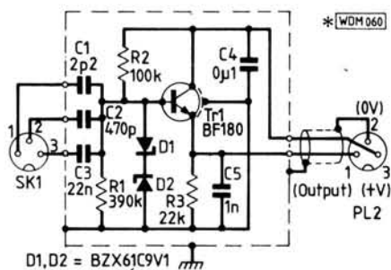
Fig. 2: Circuit diagram of probe
