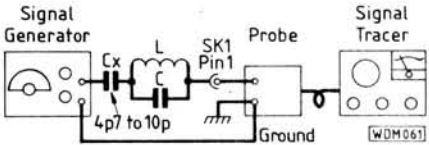
Fig. 6: Equipment layout showing probe connections used for resonance testing
